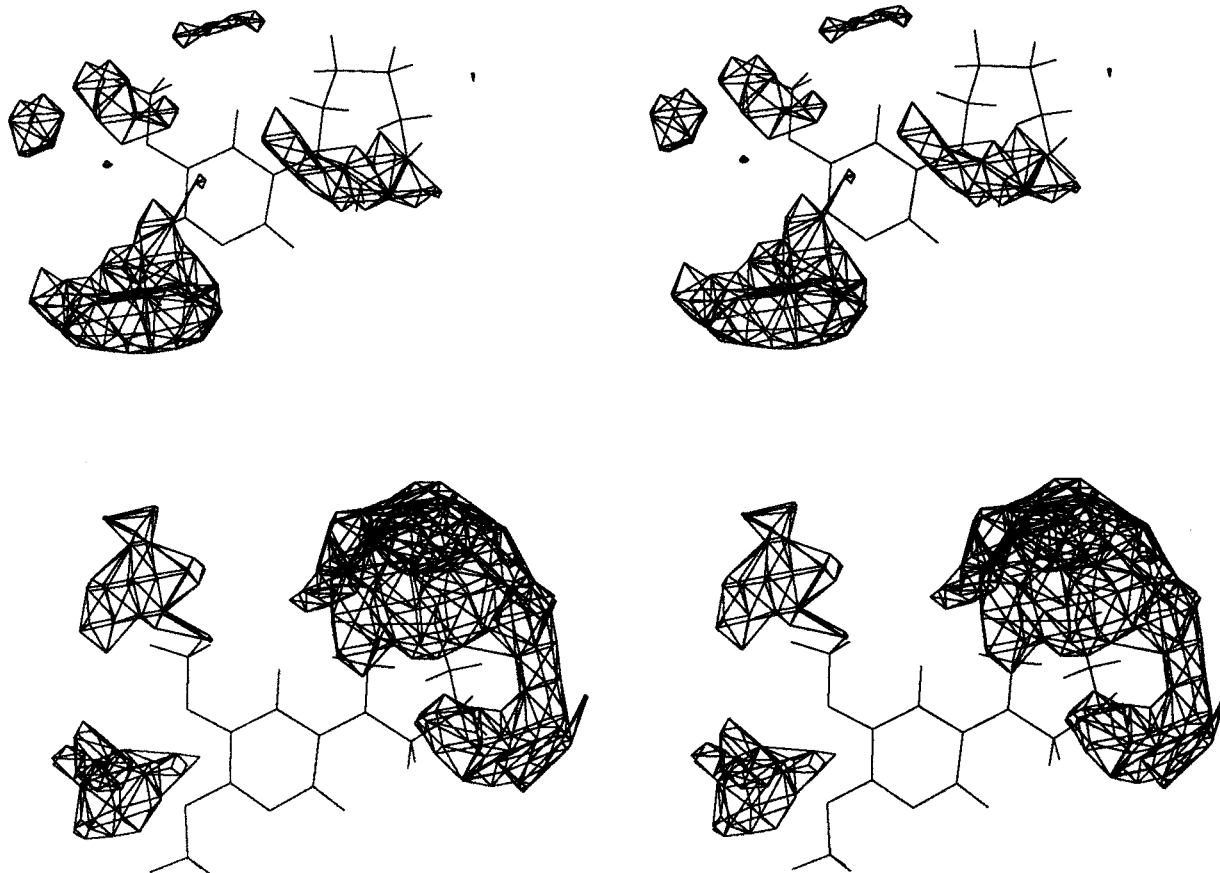
Figure 3. Contour maps (stereoview) for \alpha 4 \beta 2 nAChR affinity. The negative (top) and positive (bottom) coefficients at the 0.002 level for the OH2 probe are shown. An unfavorable interaction (positive interaction energy) between a substituent and the probe in regions with negative coefficients will decrease -\log(\text{IC}_{50}) , i.e., reduce the activity of the compound and vice versa for positive coefficients. The compound 22 is drawn to illustrate the size of the regions.
